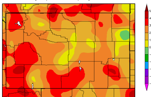
Departure from Normal Temperature (°F) 3/17/2015 – 5/15/2015
