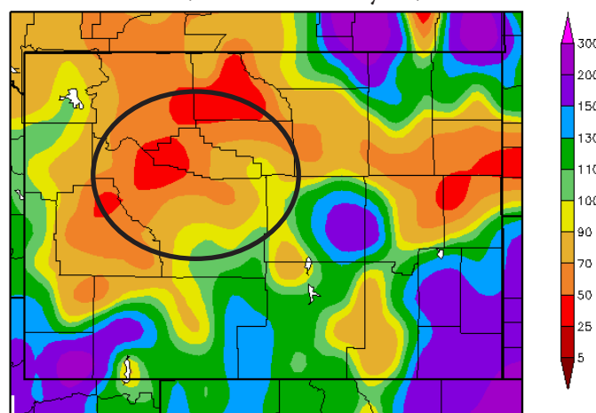
Percent of Normal Precipitation (%) December 1, 2015 - February 29, 2016
