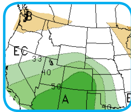
3-Month Precipitation Outlook Valid March-May 2016
