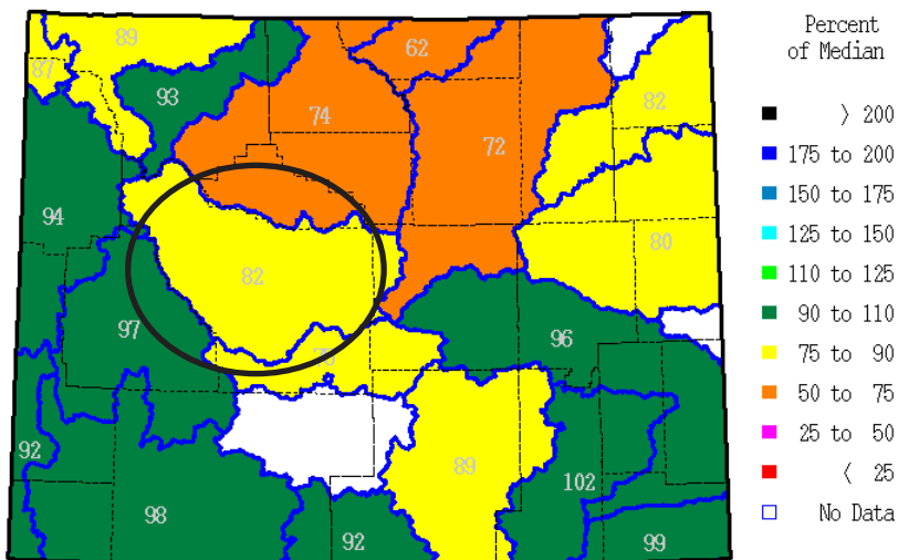
Snow Water Equivalent (SWE) % of Median by Basin and SNOTEL Site (Wyoming) as of February 29, 2016
