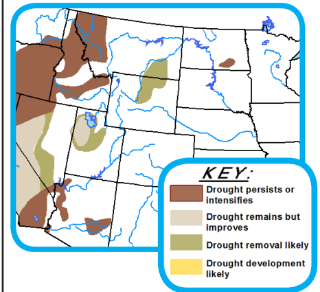
U.S. Seasonal Drought Outlook Valid February 18-May 31, 2016
