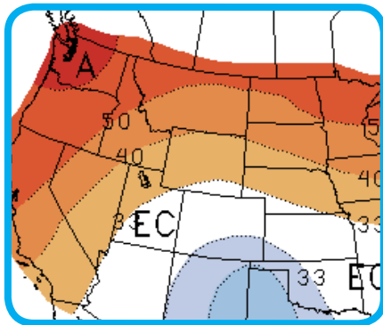
3-Month Temperature Outlook Valid March-May 2016
